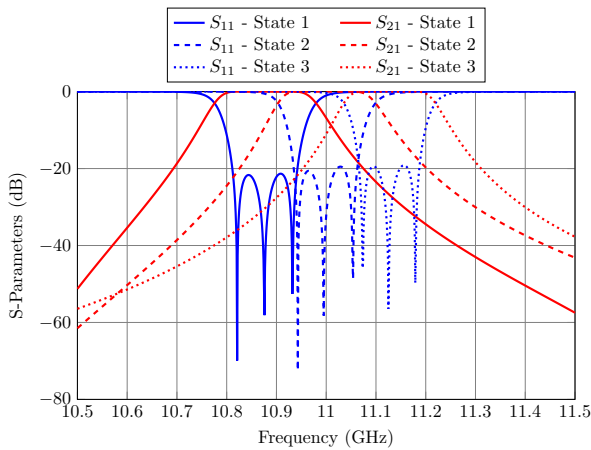
FIGURE 10. Performance of the LA filter. In order to change between the possible states, we must set the inner pins of the MTPs as shown in Fig. 3.
