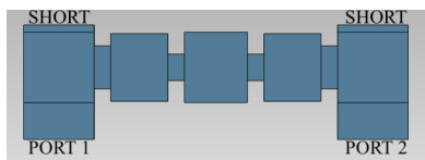
FIGURE 6. Step 1: The first filter is added to the manifold.
