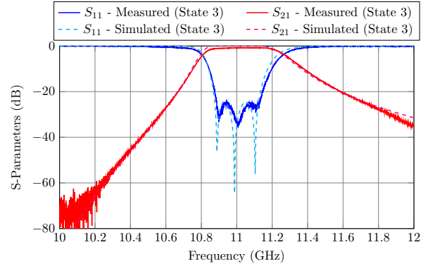
FIGURE 19. Experimental results compared to the HA model performance for the third state.
