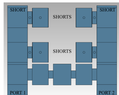
FIGURE 8. Step 3: The third channel (filter) is added to the manifold.
