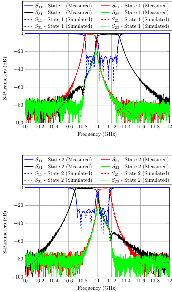
FIGURE 37. Experimental results for the state 1 (top) and state 2 (bottom) of the designed diplexer.
