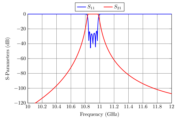
FIGURE 31. Response of the component displayed in Fig. 30.
